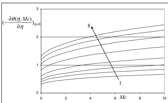
Fig. 9. Numerical results of wall temperature gradient on the plate surface, \left(-\frac{\partial \theta(\eta, Mc)}{\partial \eta}\right)_{\eta=0} varying with Prandtl number Pr and mixed convection parameter Mc (Lines 1 to 8 denote Pr = 0.3, 0.6, 1, 2, 5, 10, 15 and 20 respectively)
